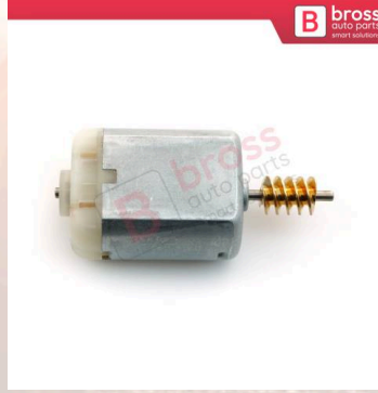
BGE675 GM Opel Chevrolet Buick W203 W209 W219 W171 W211 İçin Kapı Kilit Motoru 1020653 16 mm Şaft
